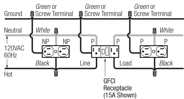
Wiring Diagram 8 GFCI Receptacle Wiring
